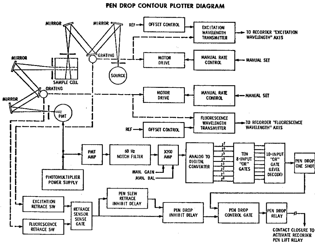
Figure 1. Schematic diagram of the electronics circuit designed to generate the isointensity contour plot. PMT: photomultiplier; Source: excitation light source
